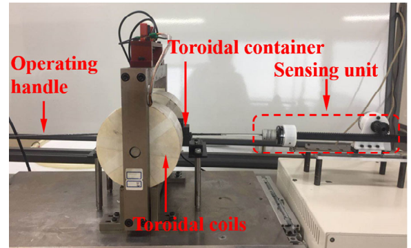
Figure 4 Master manipulator based on MR fluid (see online version for colours)
