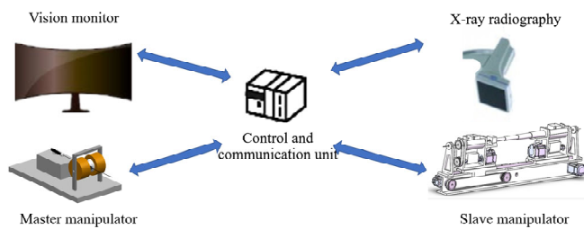
Figure 1 Conceptual diagram of the robot-assisted catheter system (see online version for colours)
