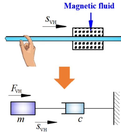
Figure 5 Mass-damper model for the tremor suppression (see online version for colours)
