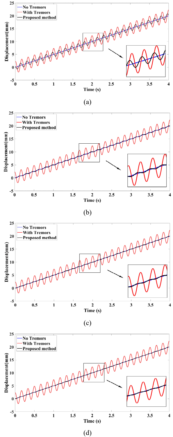
Figure 7 Results of simulation II, (a) c = 5 Pa\cdot s (b) c = 25 Pa\cdot s (c) c = 45 Pa\cdot s (d) c = 65 Pa\cdot s (see online version for colours)
