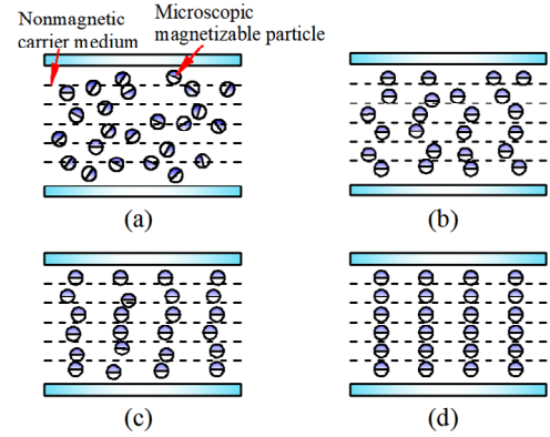
Figure 3 Particle configuration in the magnetic field with different intensities, (a) no magnetic flux (b)–(d) different configurations with the gradually increasing intensity (see online version for colours)
