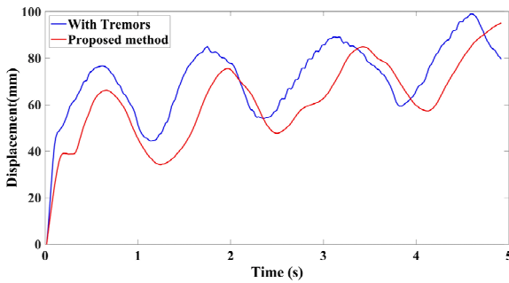
Figure 9 Results of the tremor reduction with and without the proposed method (see online version for colours)
